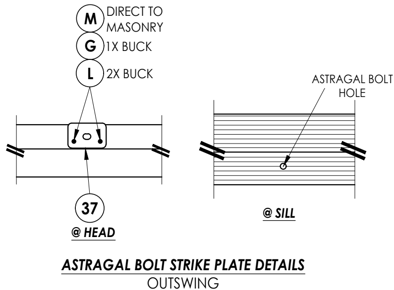
HARDWARE DETAILS
