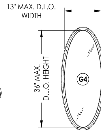
3/4 OVAL
