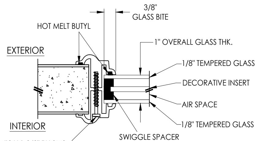
G4 GLAZING DETAIL TKI PRODUCTS LITE FRAME
