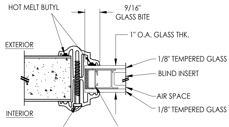
1/2 LITE w/ MICROBLINDS
